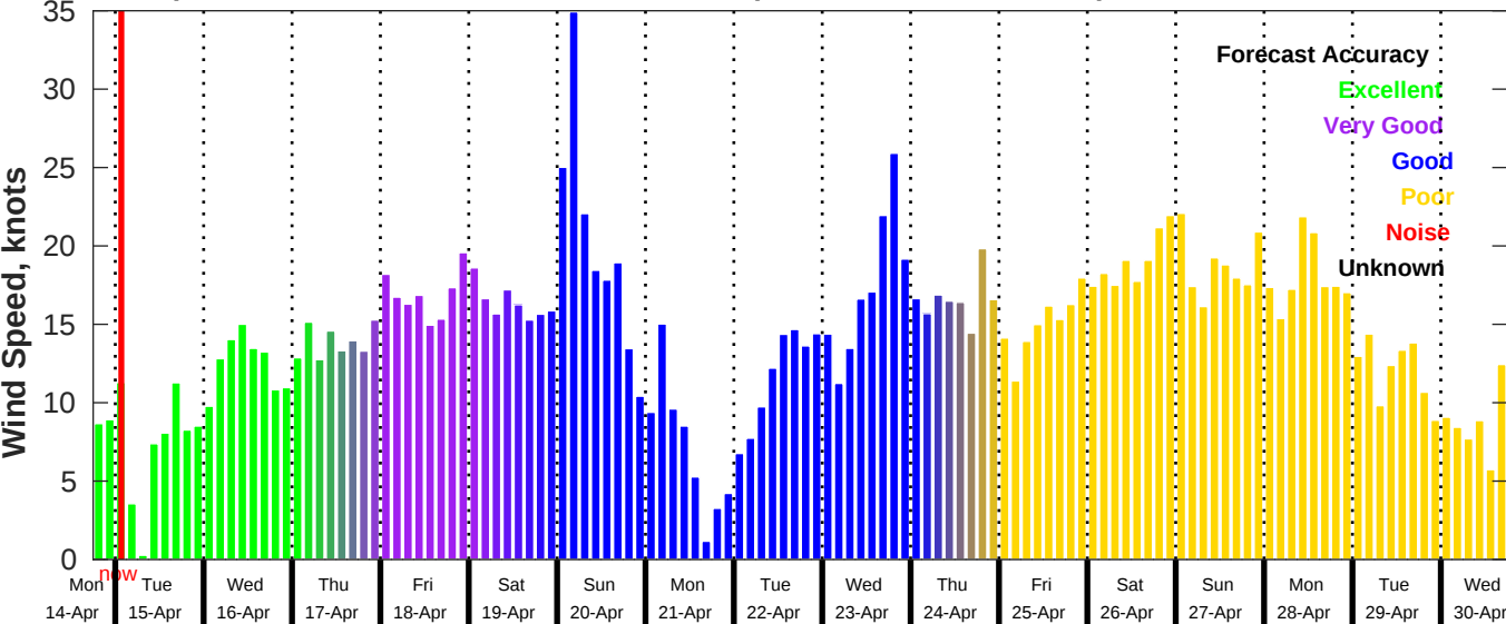
GFS Wind Speed Forecast for NDBC 42035 from 14-Apr-2025 18:00:00 to 30-Apr-2025 18:00:00
