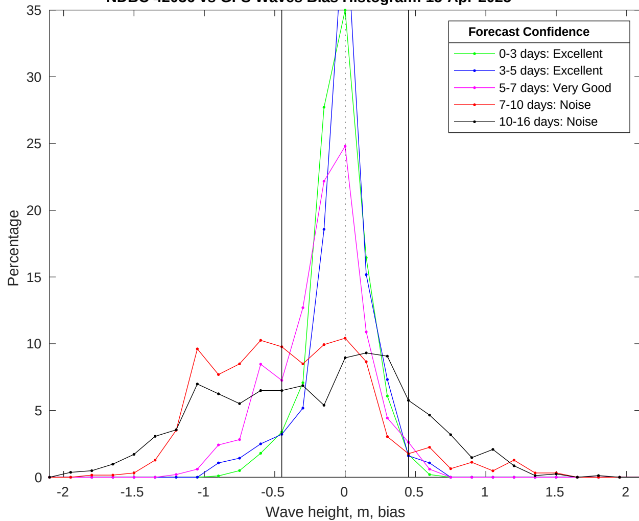
NDBC 42036 vs GFS Waves Bias Histogram: 15-Apr-2025
