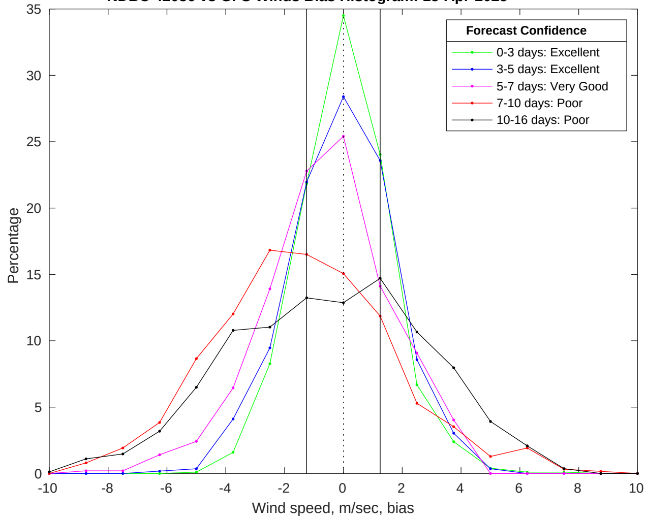
NDBC 42036 vs GFS Winds Bias Histogram: 15-Apr-2025
