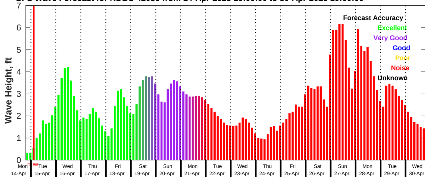
GFS Wave Forecast for NDBC 42036 from 14-Apr-2025 19:00:00 to 30-Apr-2025 19:00:00
