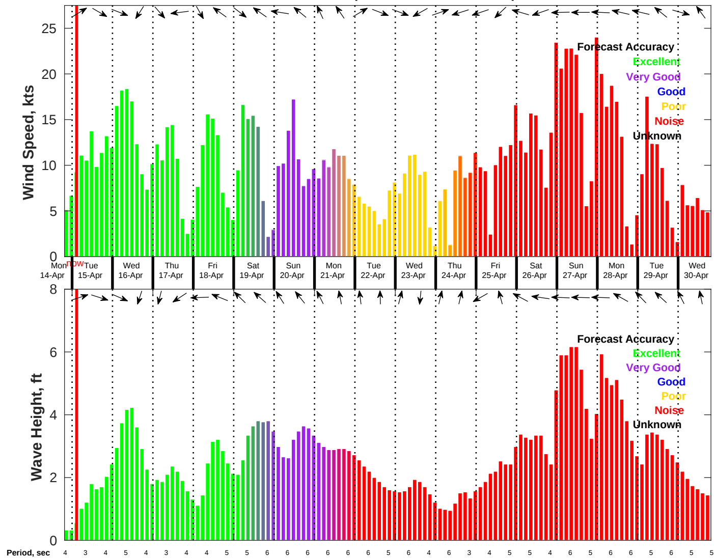
Wind & Wave Forecast for NDBC 42036 from 14-Apr-2025 19:00:00 to 30-Apr-2025 19:00:00
