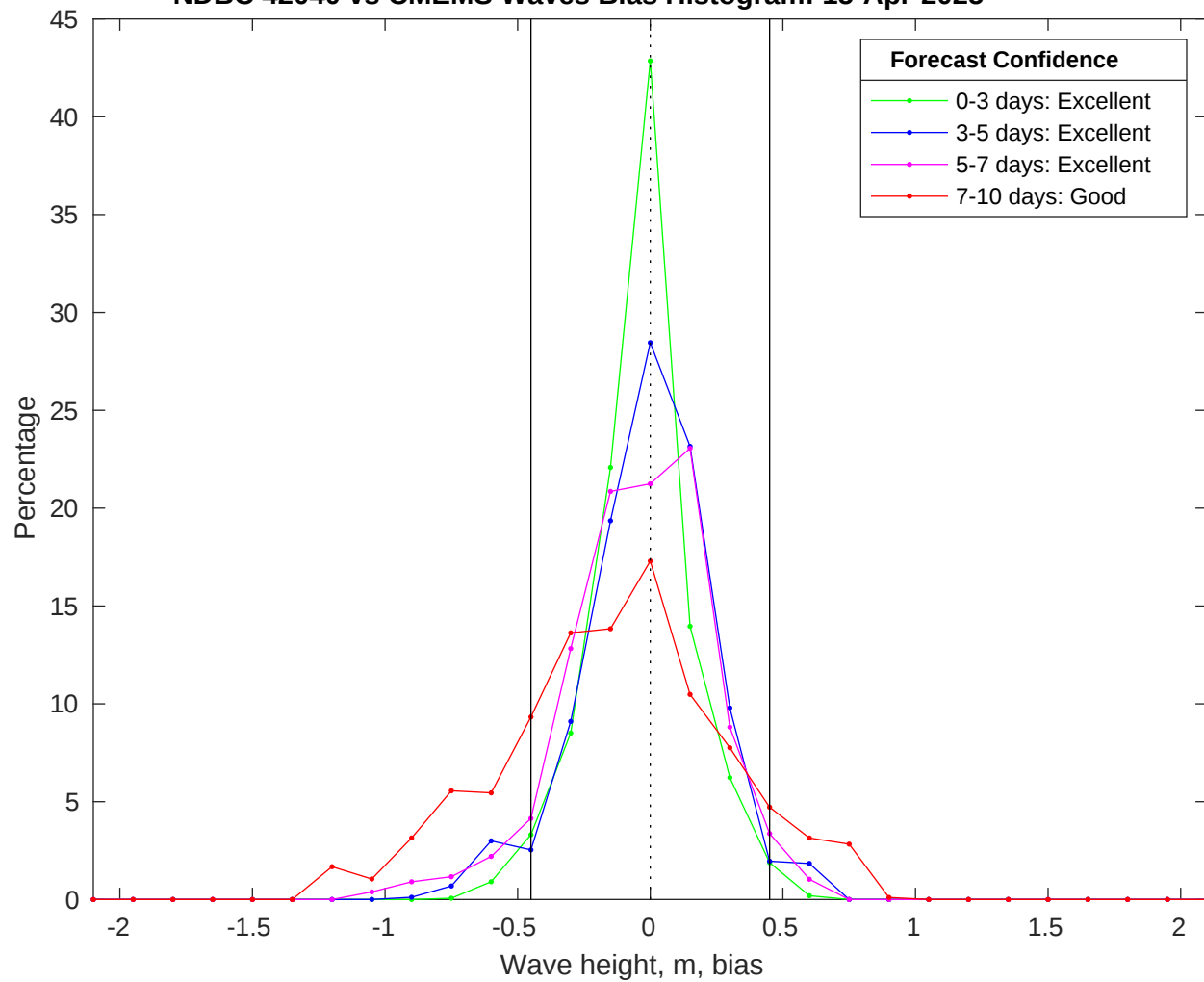
NDBC 42040 vs CMEMS Waves Bias Histogram: 15-Apr-2025
