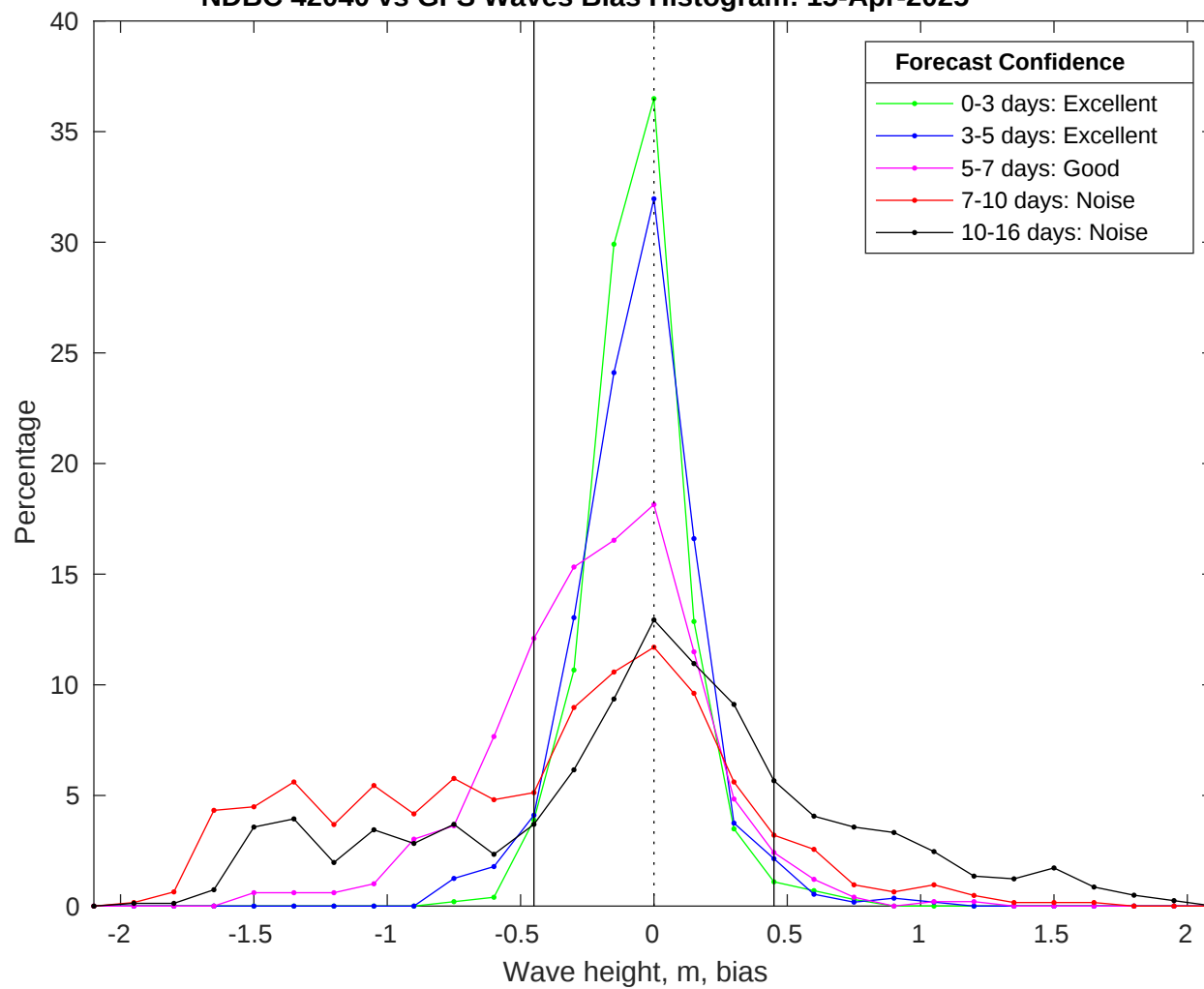
NDBC 42040 vs GFS Waves Bias Histogram: 15-Apr-2025
