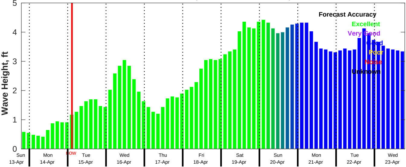
CMEMS Wave Forecast for NDBC 42040 from 13-Apr-2025 19:00:00 to 23-Apr-2025 19:00:00
