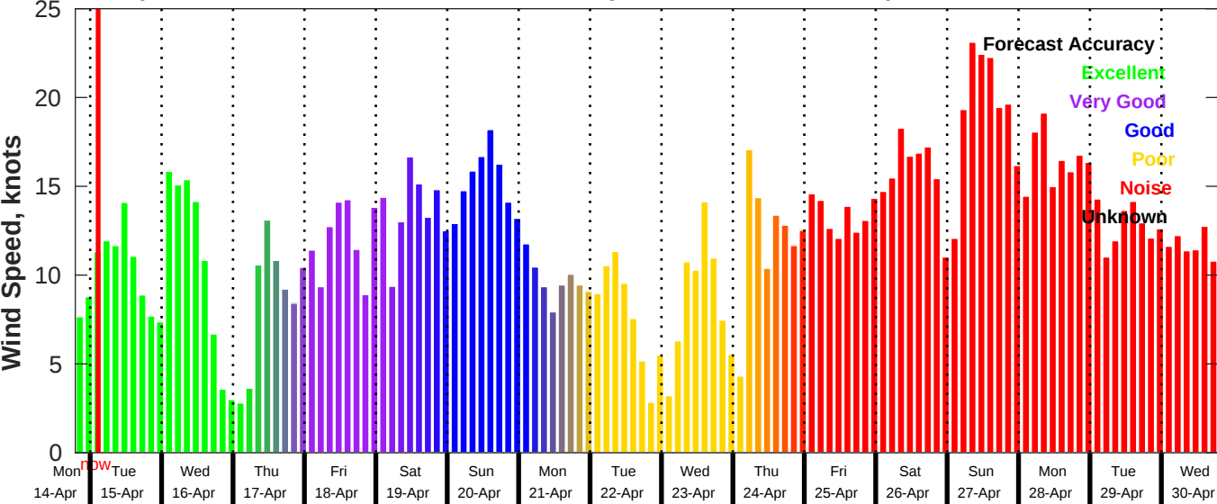
GFS Wind Speed Forecast for NDBC 42040 from 14-Apr-2025 19:00:00 to 30-Apr-2025 19:00:00
