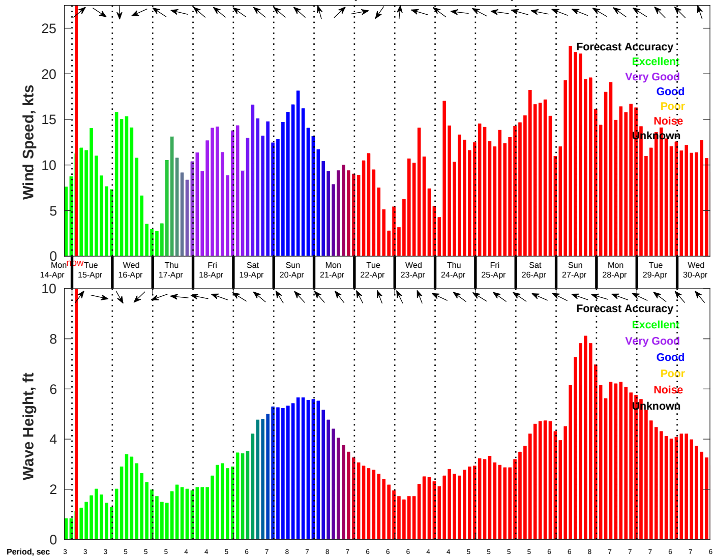
Wind & Wave Forecast for NDBC 42040 from 14-Apr-2025 19:00:00 to 30-Apr-2025 19:00:00
