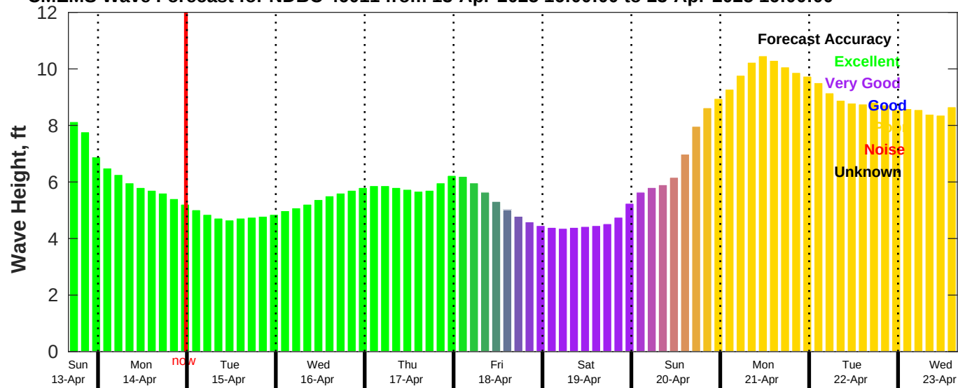
CMEMS Wave Forecast for NDBC 46011 from 13-Apr-2025 16:00:00 to 23-Apr-2025 16:00:00
