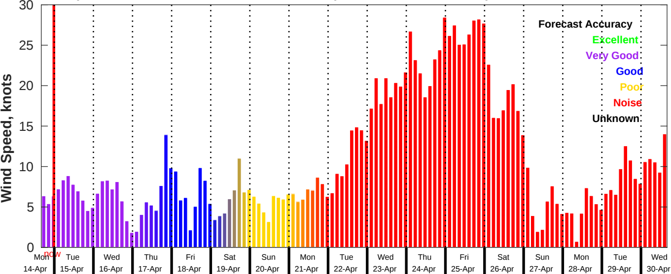
GFS Wind Speed Forecast for NDBC 46011 from 14-Apr-2025 16:00:00 to 30-Apr-2025 16:00:00
