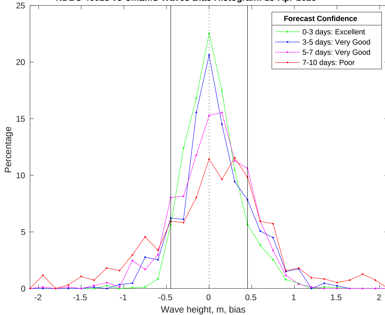
NDBC 46028 vs CMEMS Waves Bias Histogram: 15-Apr-2025
