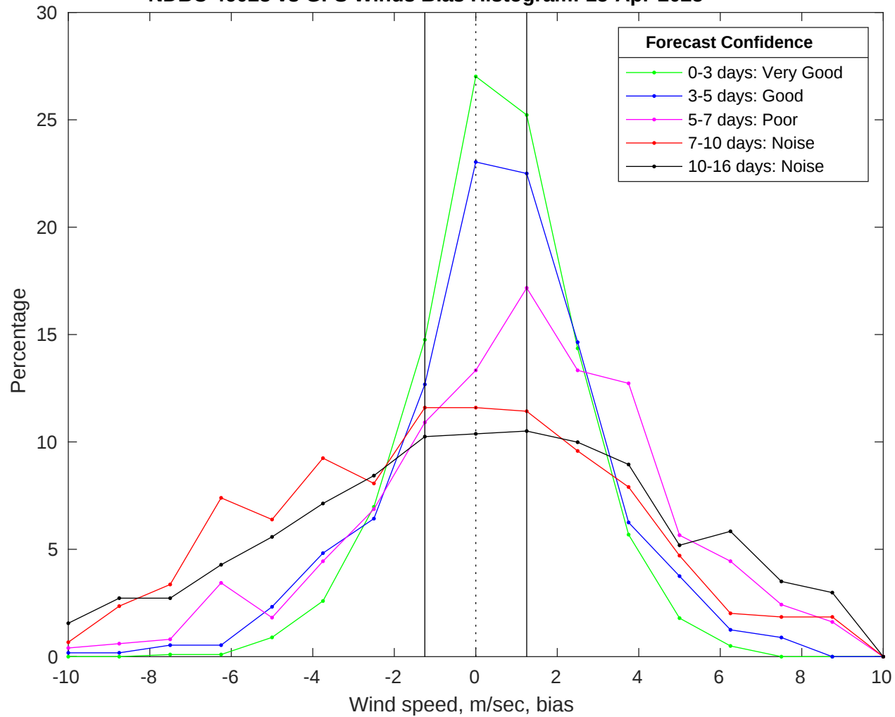
NDBC 46028 vs GFS Winds Bias Histogram: 15-Apr-2025
