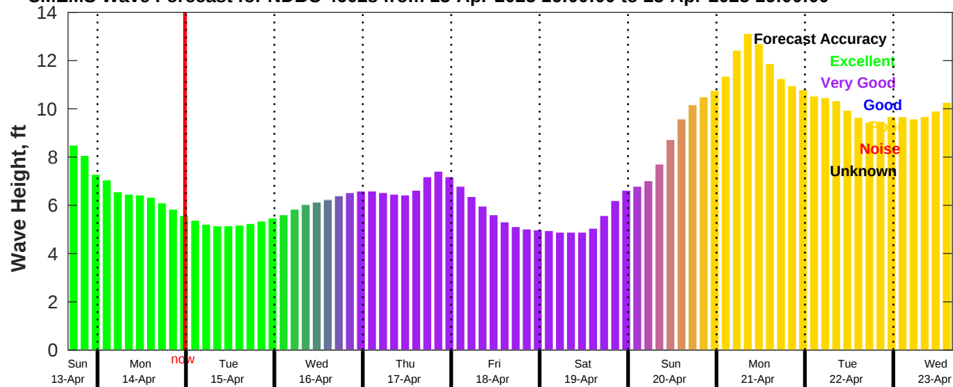
CMEMS Wave Forecast for NDBC 46028 from 13-Apr-2025 16:00:00 to 23-Apr-2025 16:00:00
