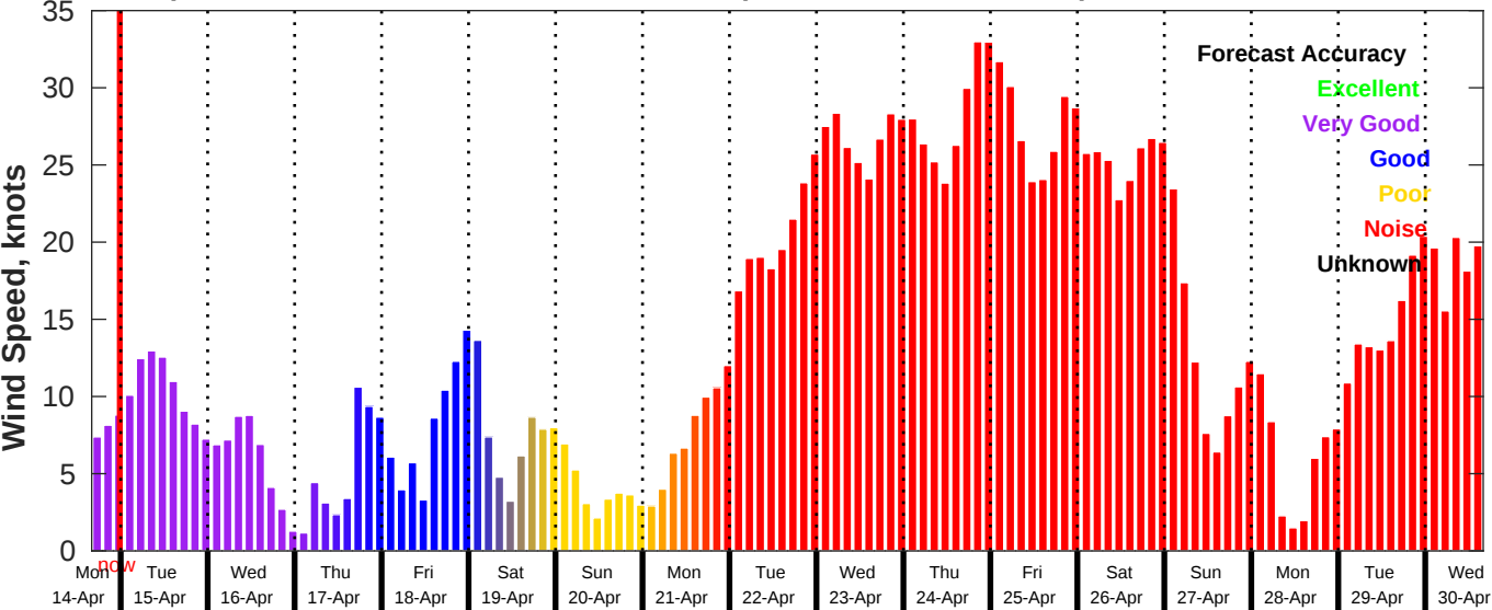
GFS Wind Speed Forecast for NDBC 46028 from 14-Apr-2025 16:00:00 to 30-Apr-2025 16:00:00
