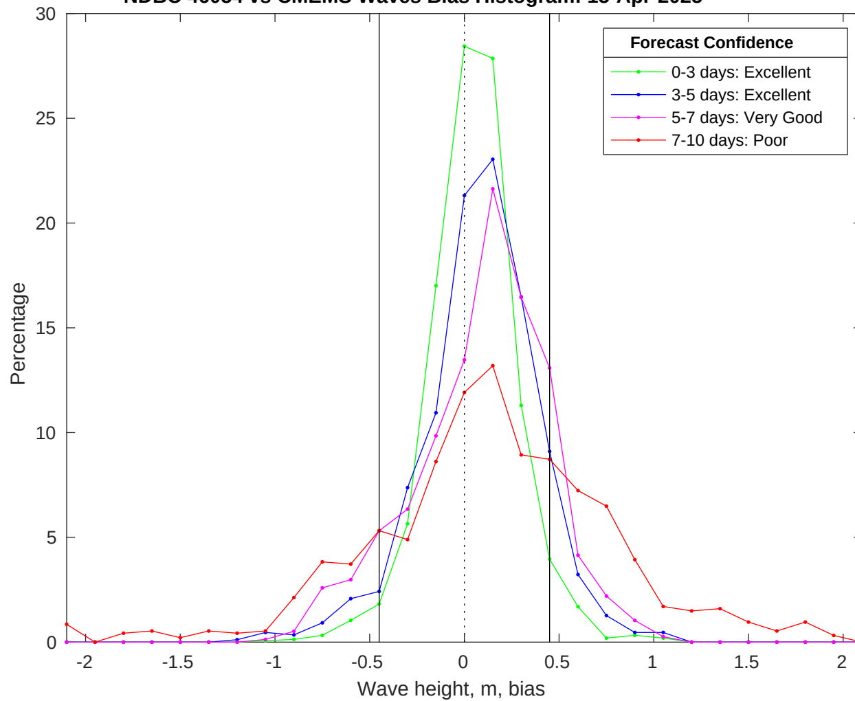
NDBC 46054 vs CMEMS Waves Bias Histogram: 15-Apr-2025
