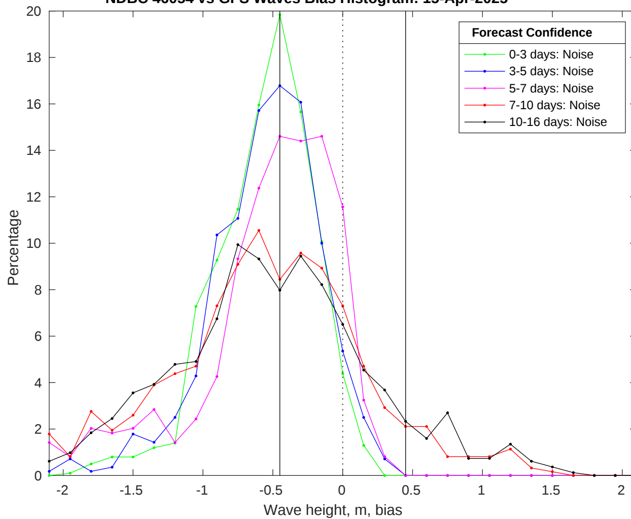
NDBC 46054 vs GFS Waves Bias Histogram: 15-Apr-2025
