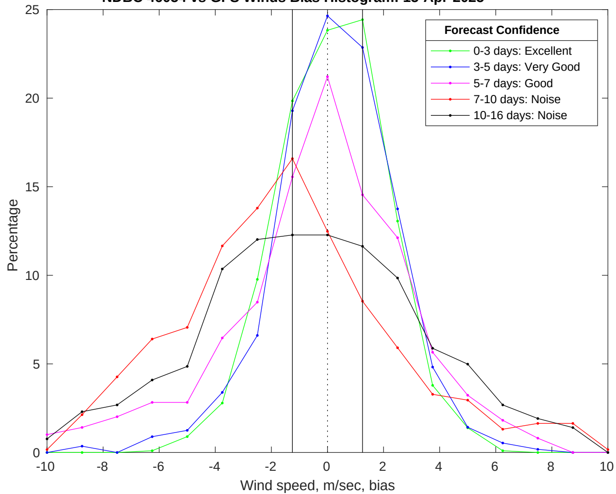
NDBC 46054 vs GFS Winds Bias Histogram: 15-Apr-2025
