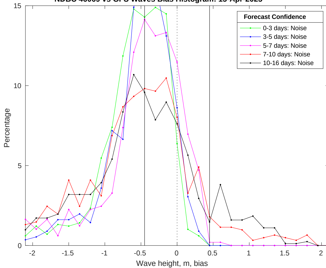
NDBC 46069 vs GFS Waves Bias Histogram: 15-Apr-2025
