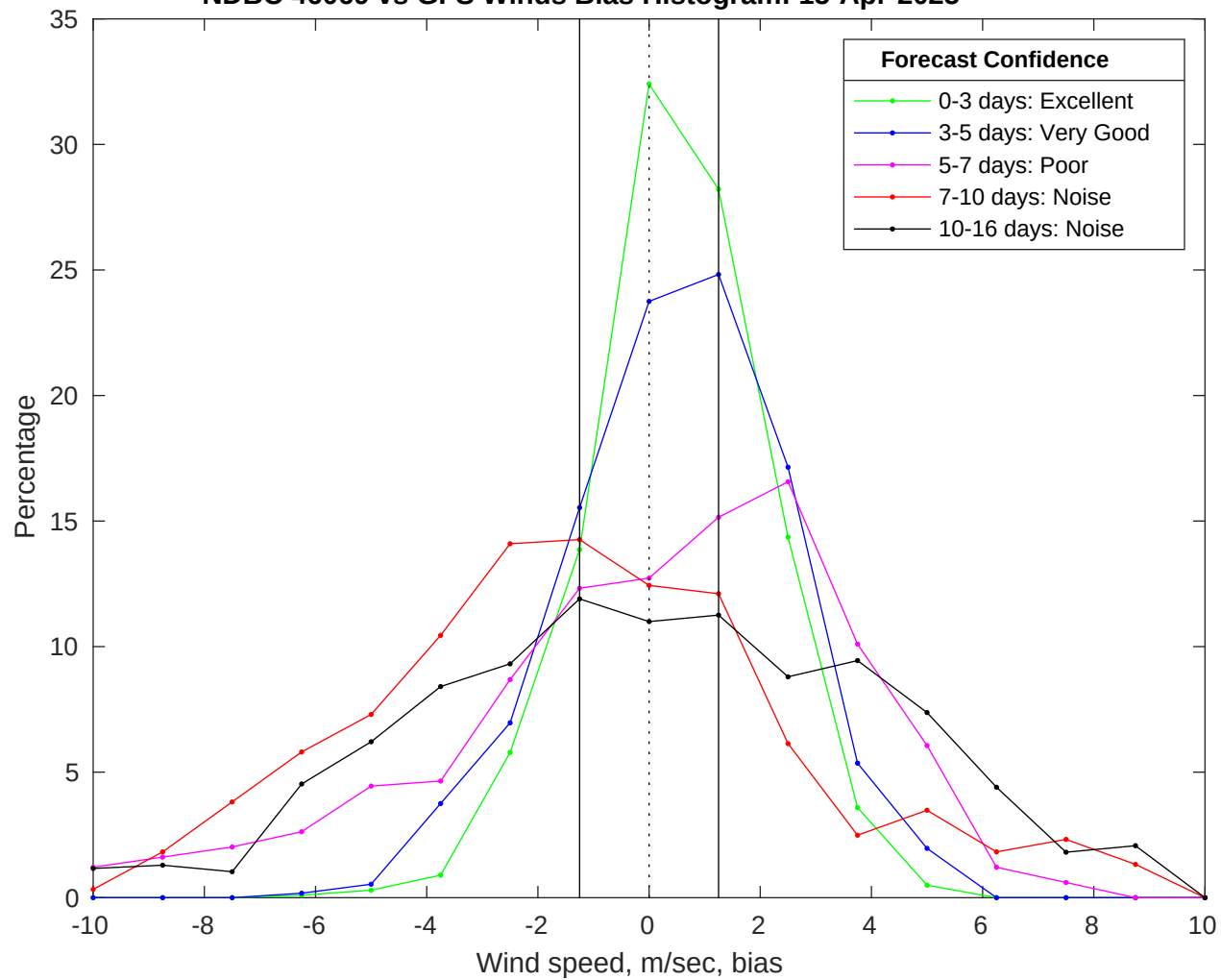
NDBC 46069 vs GFS Winds Bias Histogram: 15-Apr-2025
