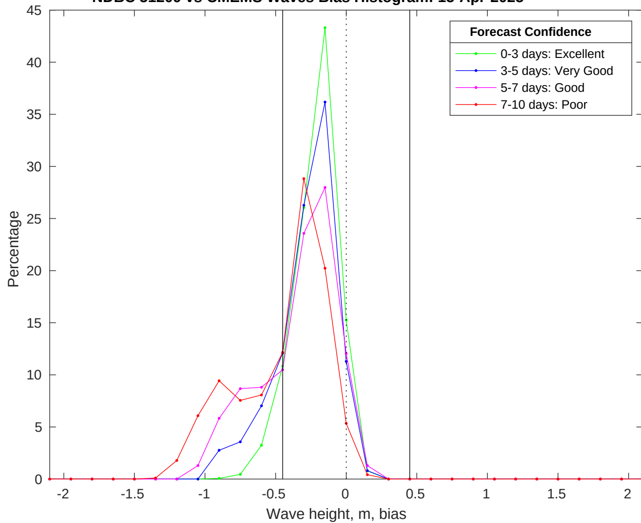
NDBC 51209 vs CMEMS Waves Bias Histogram: 15-Apr-2025
