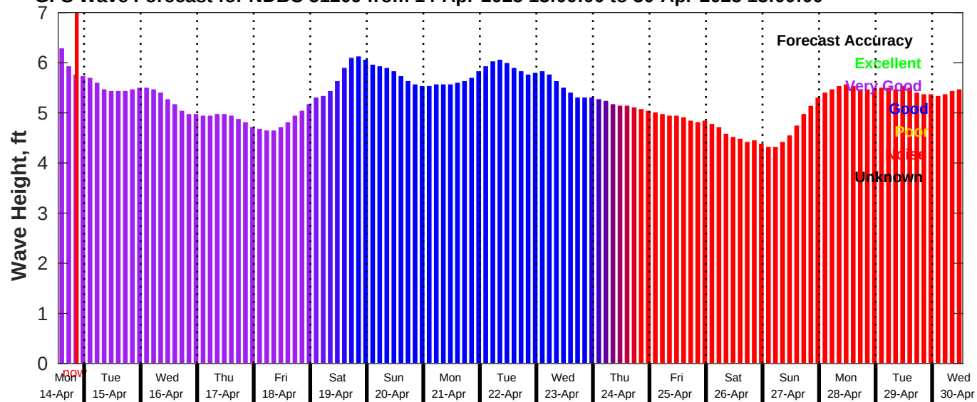
GFS Wave Forecast for NDBC 51209 from 14-Apr-2025 13:00:00 to 30-Apr-2025 13:00:00
