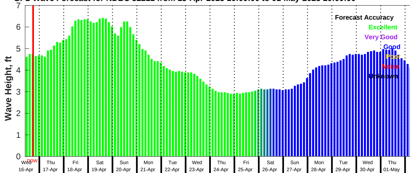
GFS Wave Forecast for NDBC 52211 from 15-Apr-2025 10:00:00 to 01-May-2025 10:00:00
