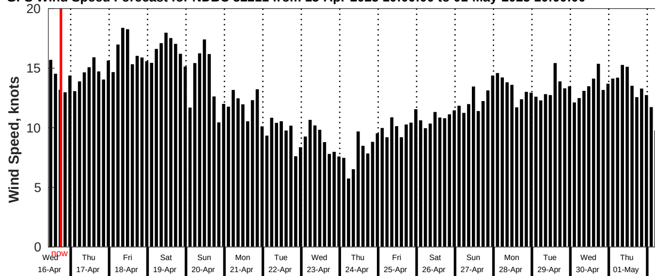
GFS Wind Speed Forecast for NDBC 52211 from 15-Apr-2025 10:00:00 to 01-May-2025 10:00:00
