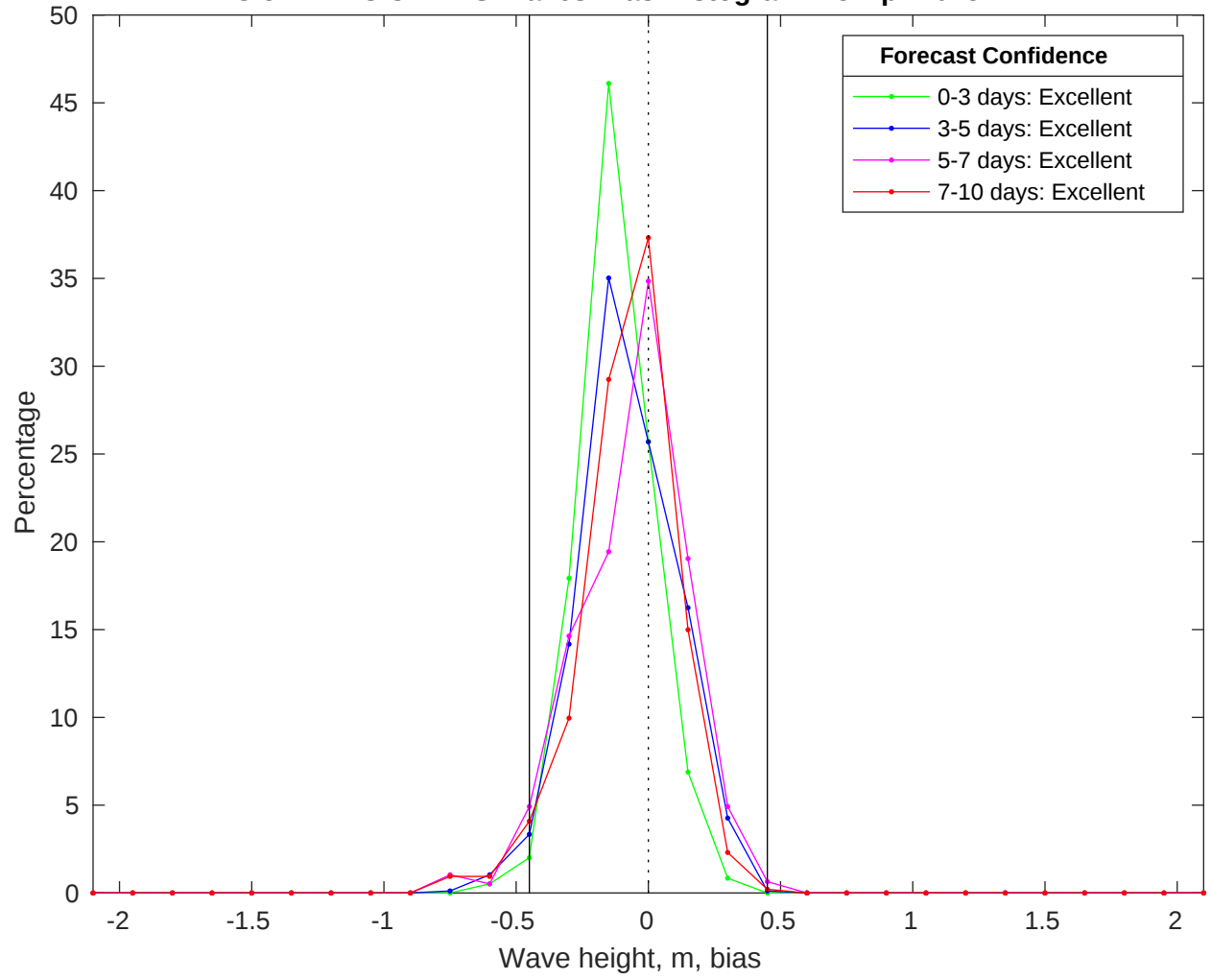
NDBC 52212 vs CMEMS Waves Bias Histogram: 15-Apr-2025
