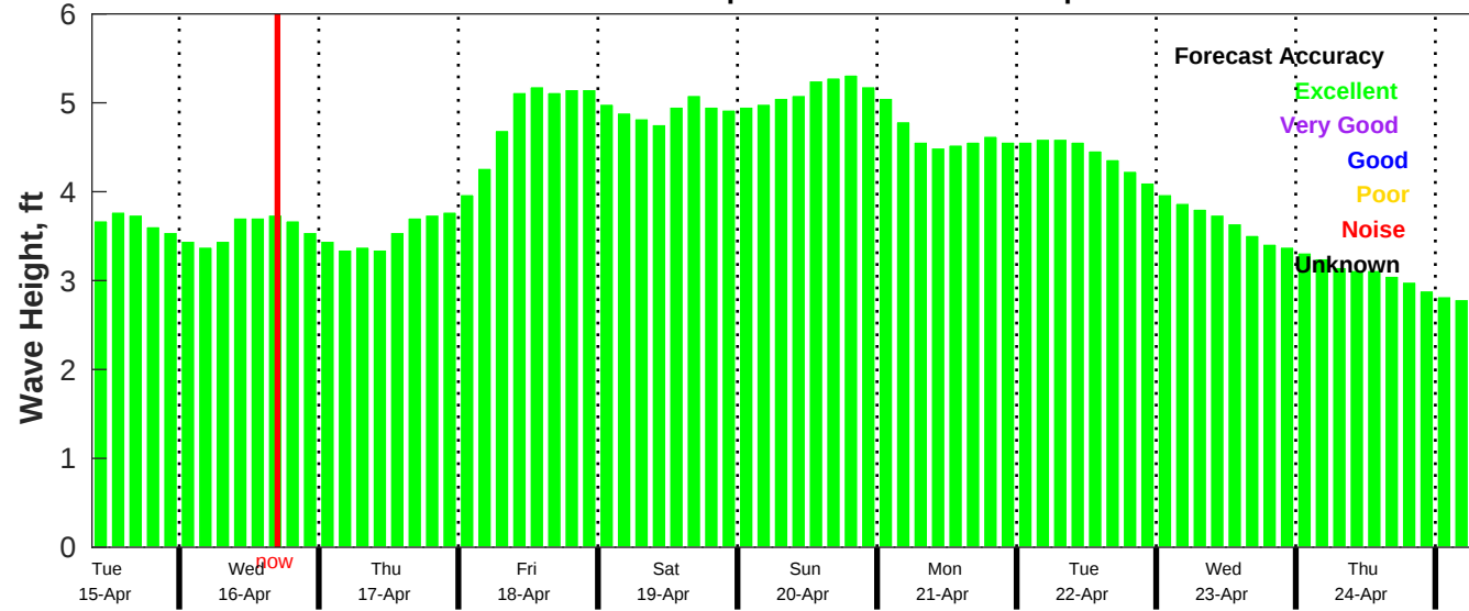
CMEMS Wave Forecast for NDBC 52212 from 14-Apr-2025 09:00:00 to 24-Apr-2025 09:00:00
