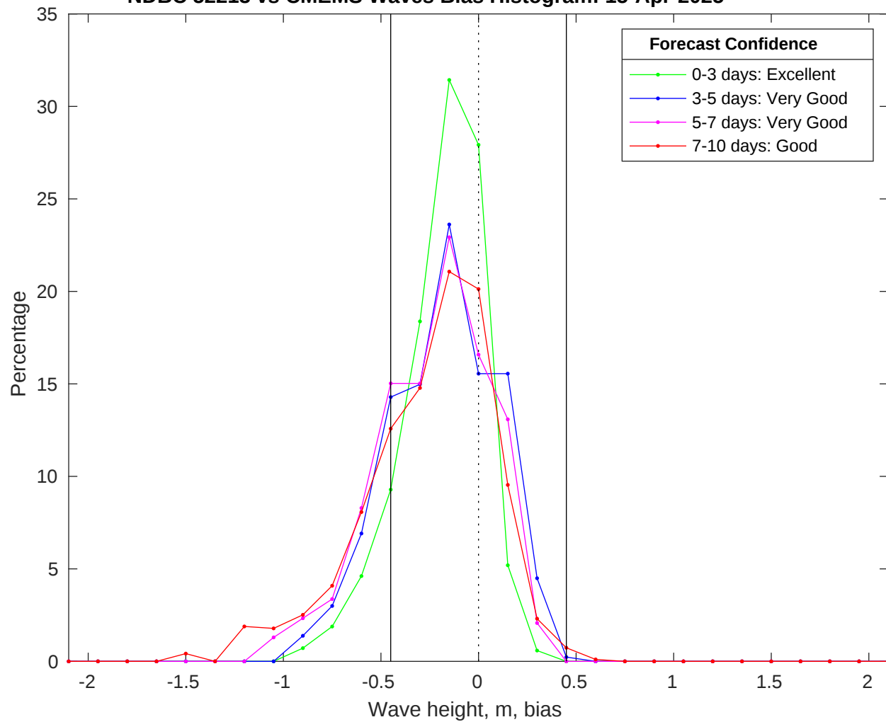
NDBC 52213 vs CMEMS Waves Bias Histogram: 15-Apr-2025
