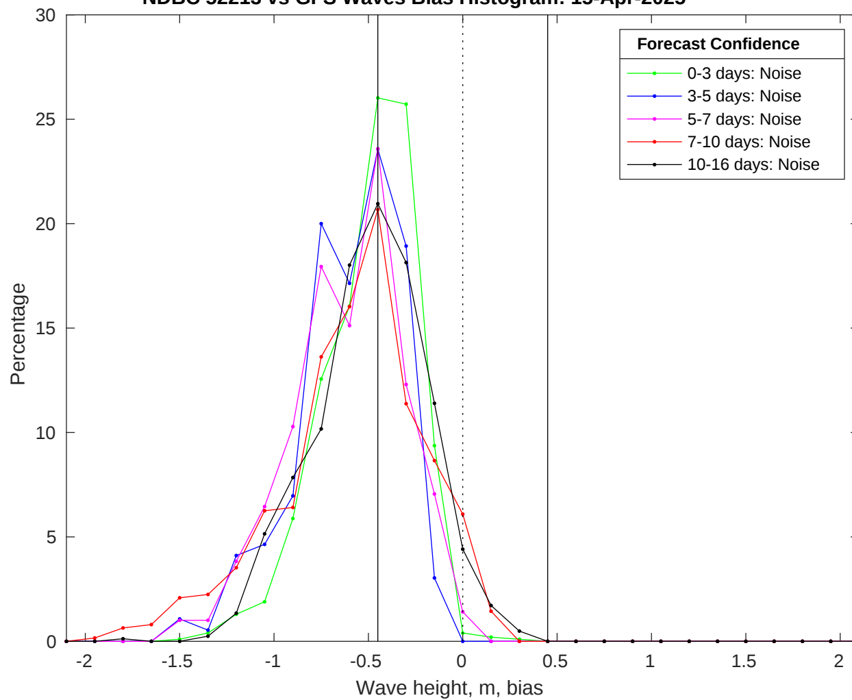
NDBC 52213 vs GFS Waves Bias Histogram: 15-Apr-2025
