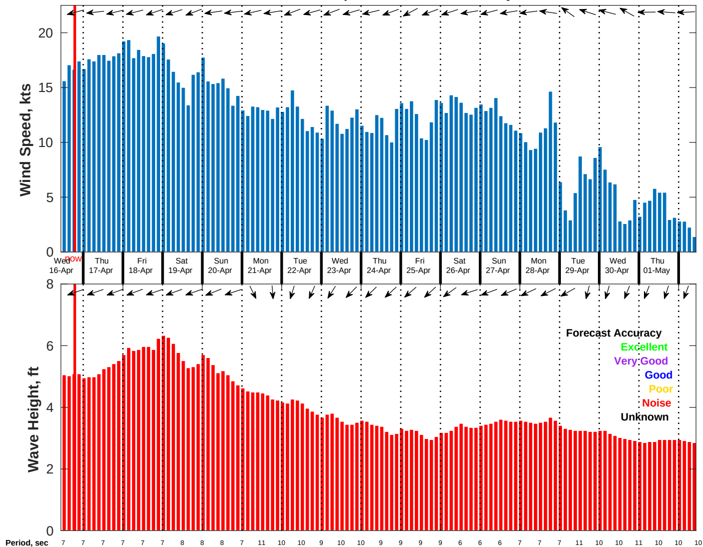
Wind & Wave Forecast for NDBC 52213 from 15-Apr-2025 11:00:00 to 01-May-2025 11:00:00
