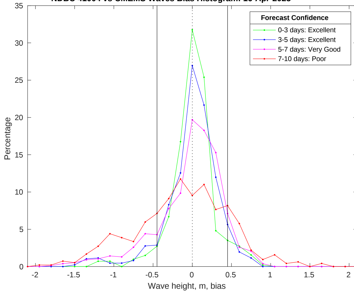
NDBC 41004 vs CMEMS Waves Bias Histogram: 16-Apr-2025
