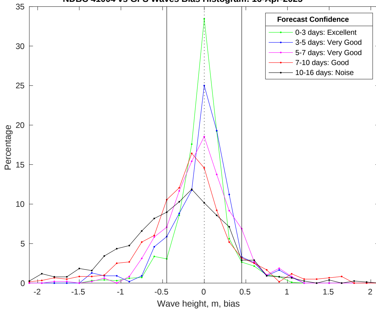
NDBC 41004 vs GFS Waves Bias Histogram: 16-Apr-2025
