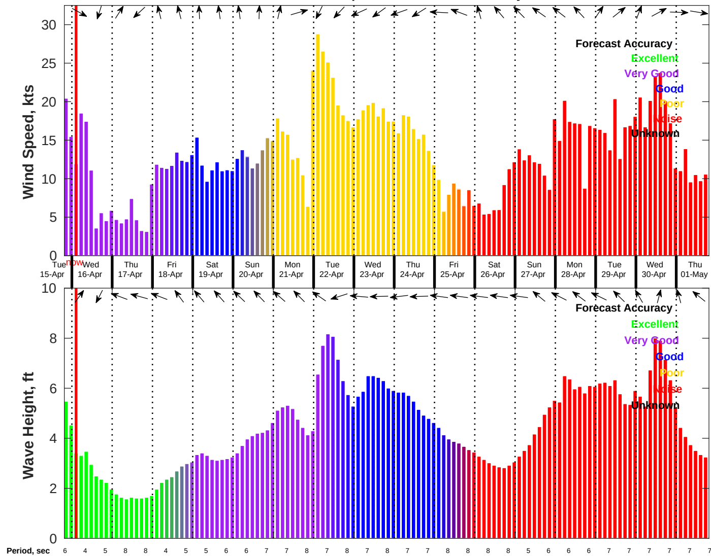
Wind & Wave Forecast for NDBC 41004 from 15-Apr-2025 19:00:00 to 01-May-2025 19:00:00
