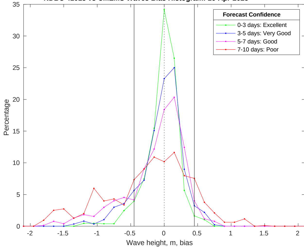
NDBC 41013 vs CMEMS Waves Bias Histogram: 16-Apr-2025
