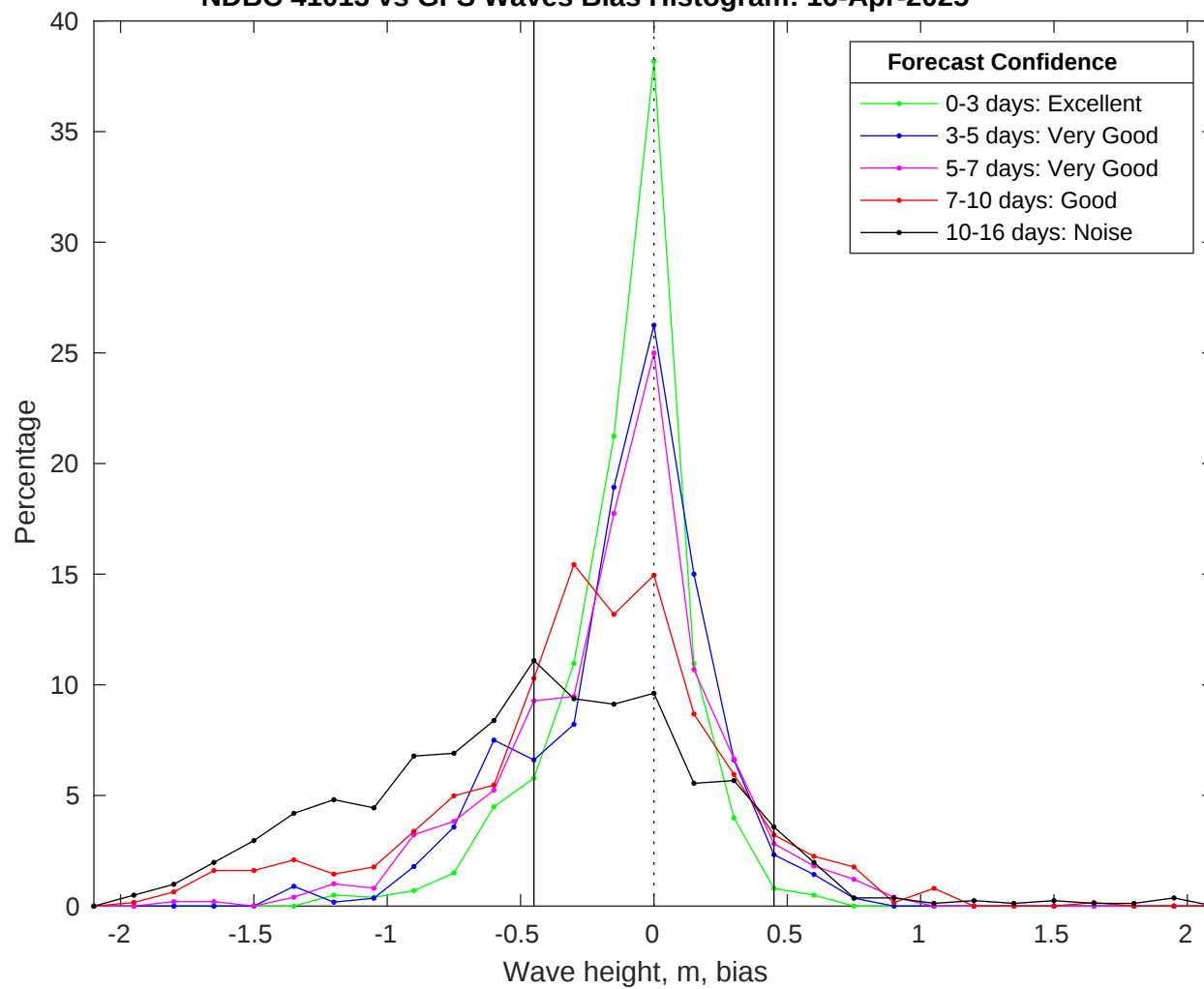
NDBC 41013 vs GFS Waves Bias Histogram: 16-Apr-2025
