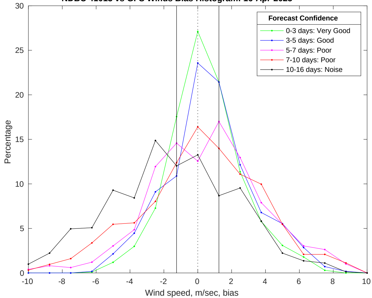
NDBC 41013 vs GFS Winds Bias Histogram: 16-Apr-2025
