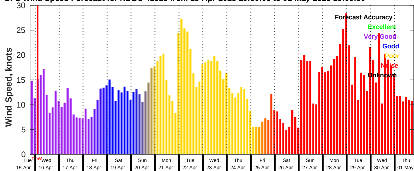
GFS Wind Speed Forecast for NDBC 41013 from 15-Apr-2025 19:00:00 to 01-May-2025 19:00:00
