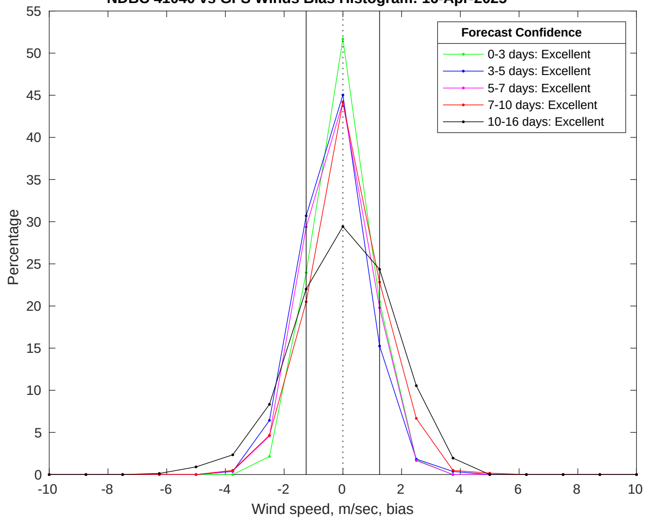
NDBC 41040 vs GFS Winds Bias Histogram: 16-Apr-2025
