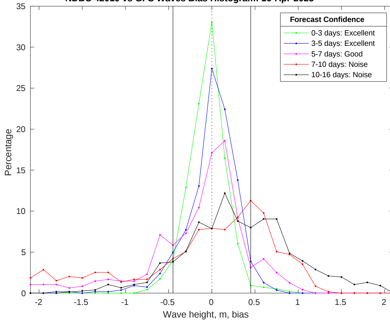
NDBC 42019 vs GFS Waves Bias Histogram: 16-Apr-2025
