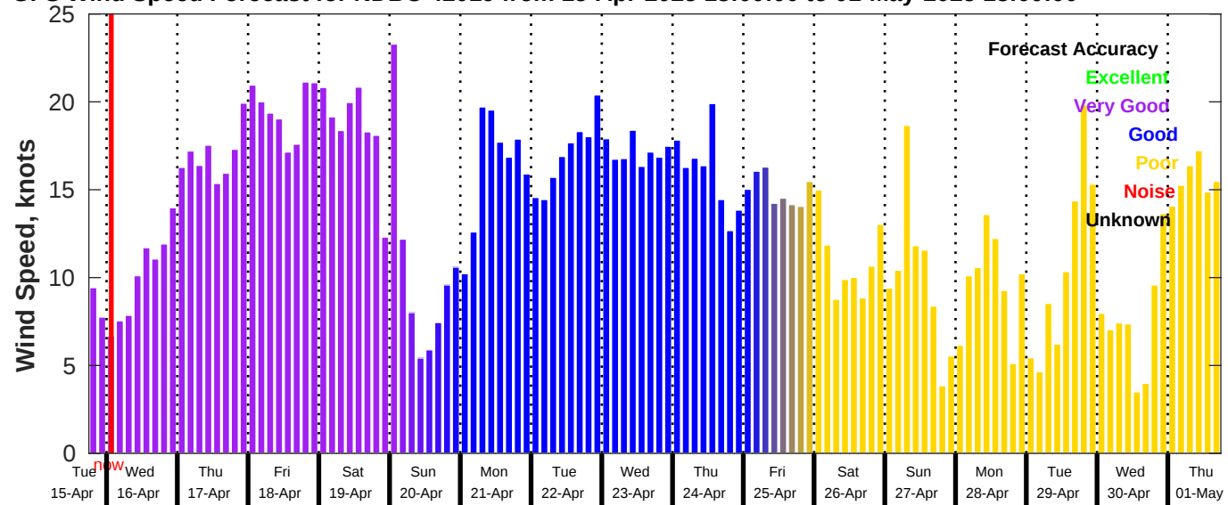
GFS Wind Speed Forecast for NDBC 42019 from 15-Apr-2025 18:00:00 to 01-May-2025 18:00:00
