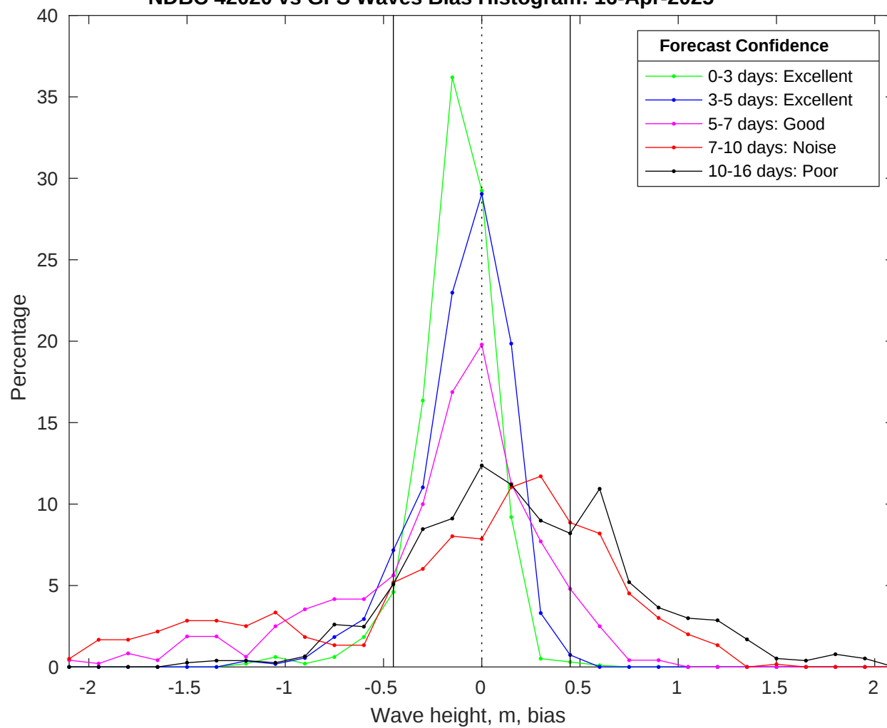
NDBC 42020 vs GFS Waves Bias Histogram: 16-Apr-2025
