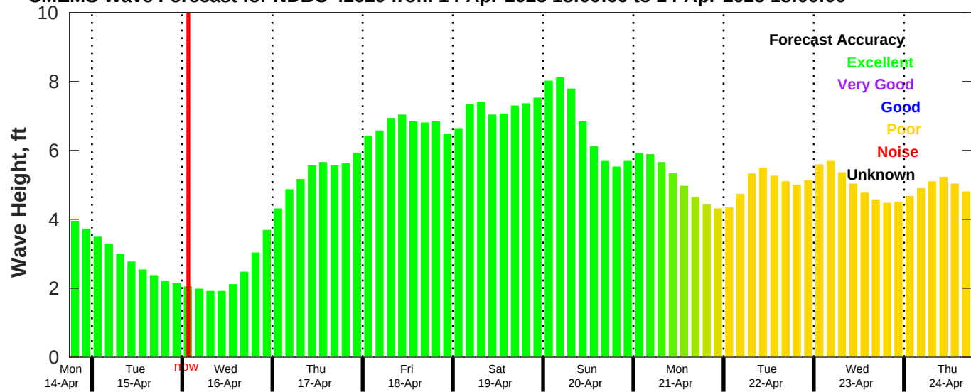
CMEMS Wave Forecast for NDBC 42020 from 14-Apr-2025 18:00:00 to 24-Apr-2025 18:00:00
