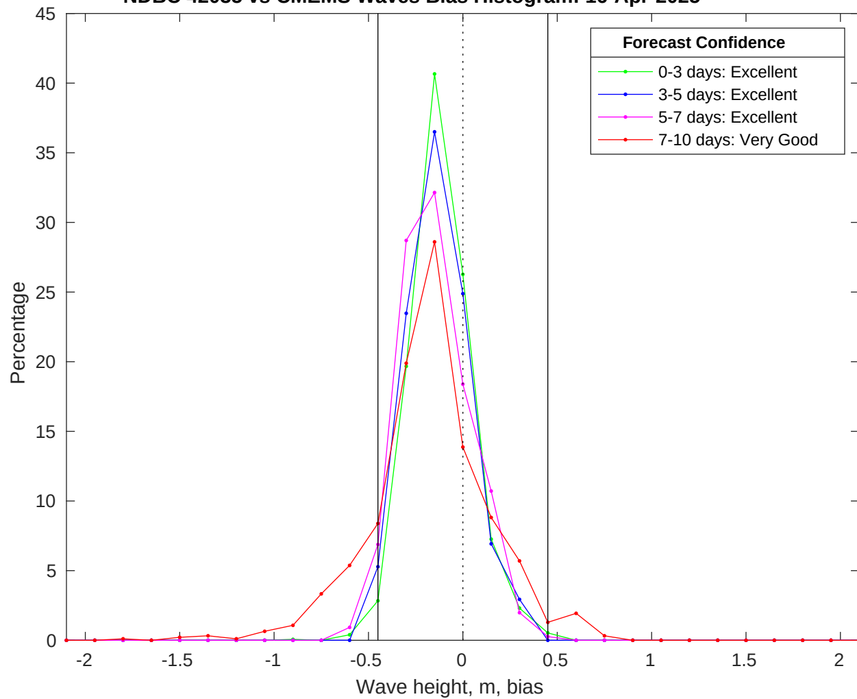
NDBC 42035 vs CMEMS Waves Bias Histogram: 16-Apr-2025
