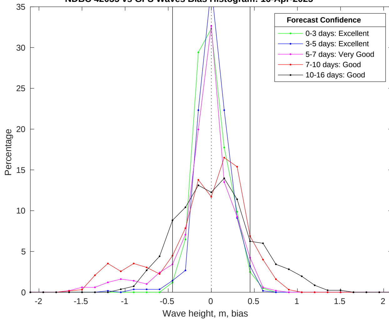
NDBC 42035 vs GFS Waves Bias Histogram: 16-Apr-2025
