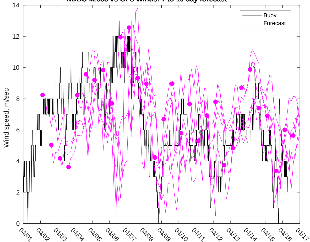
NDBC 42035 vs GFS Winds: 7 to 10 day forecast
