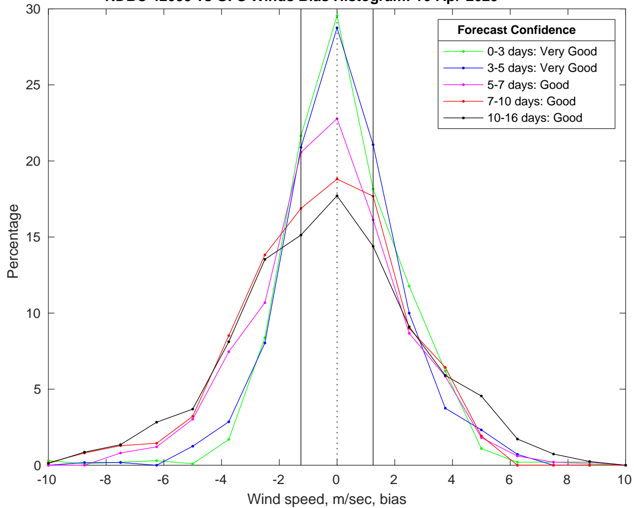
NDBC 42035 vs GFS Winds Bias Histogram: 16-Apr-2025
