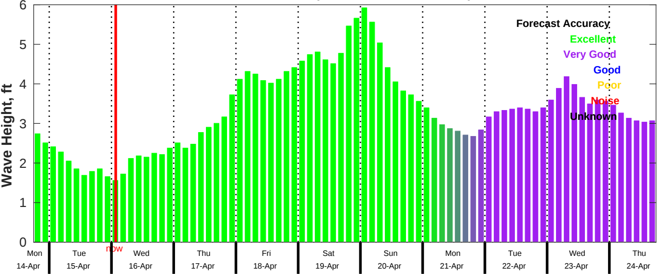
CMEMS Wave Forecast for NDBC 42035 from 14-Apr-2025 18:00:00 to 24-Apr-2025 18:00:00
