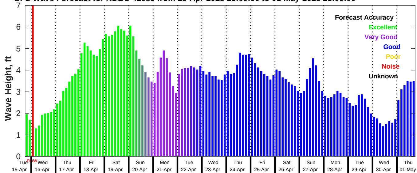
GFS Wave Forecast for NDBC 42035 from 15-Apr-2025 18:00:00 to 01-May-2025 18:00:00
