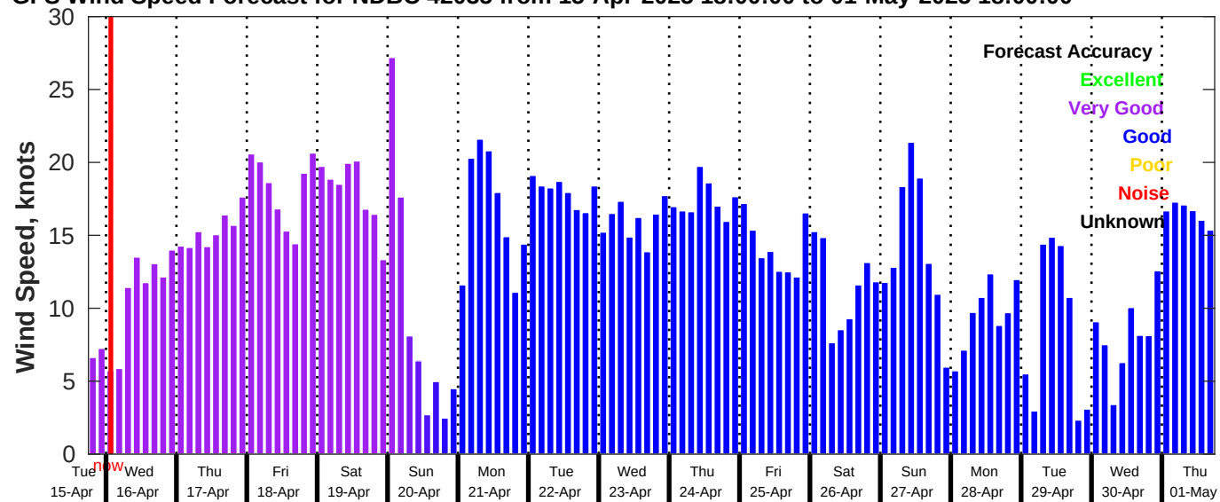
GFS Wind Speed Forecast for NDBC 42035 from 15-Apr-2025 18:00:00 to 01-May-2025 18:00:00
