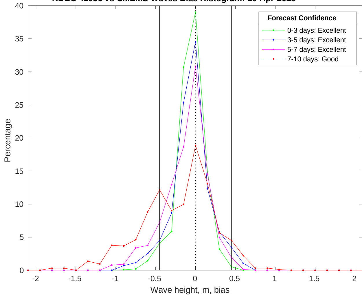
NDBC 42036 vs CMEMS Waves Bias Histogram: 16-Apr-2025
